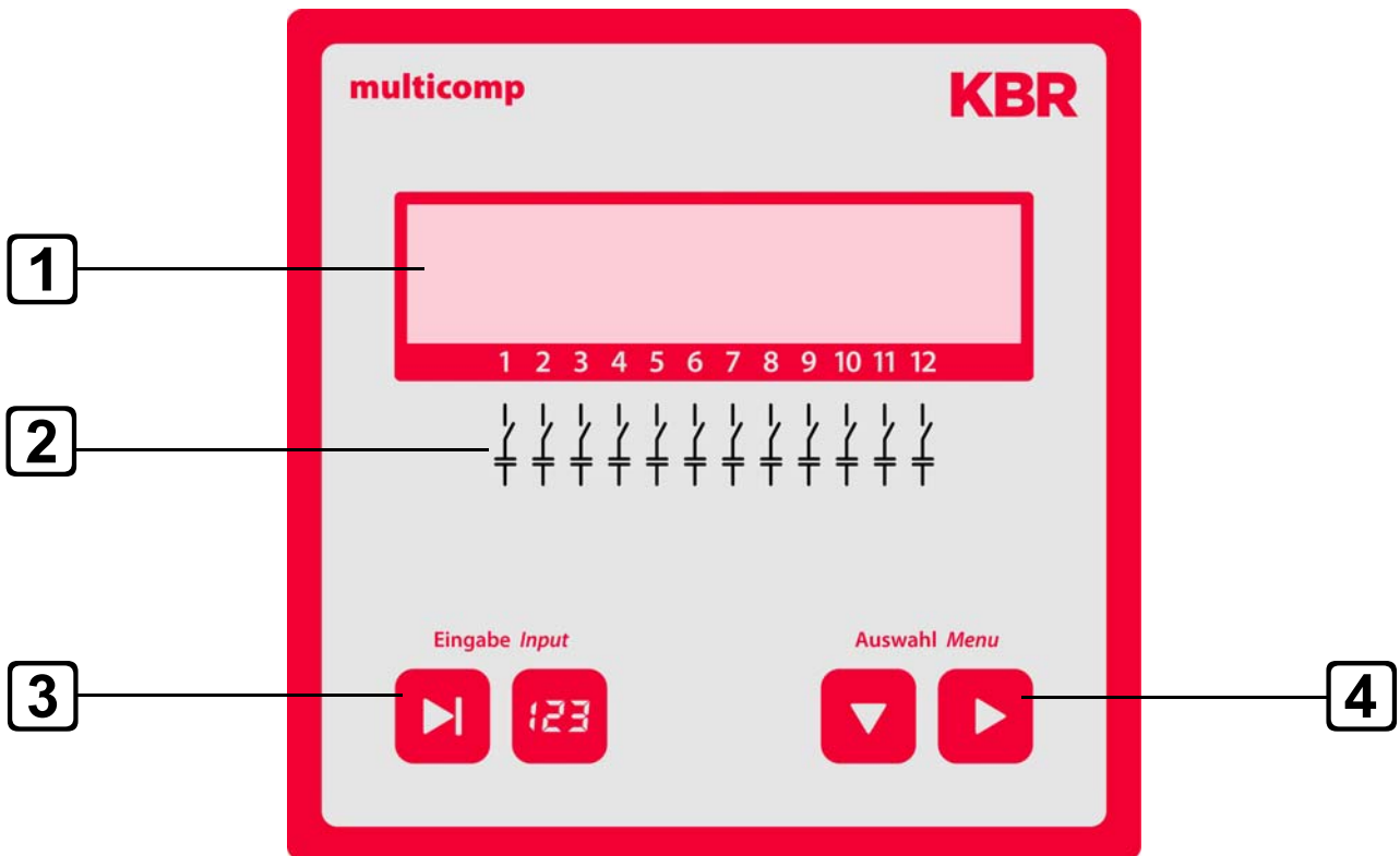
multicom 2F144-NC-1V1C12DO
