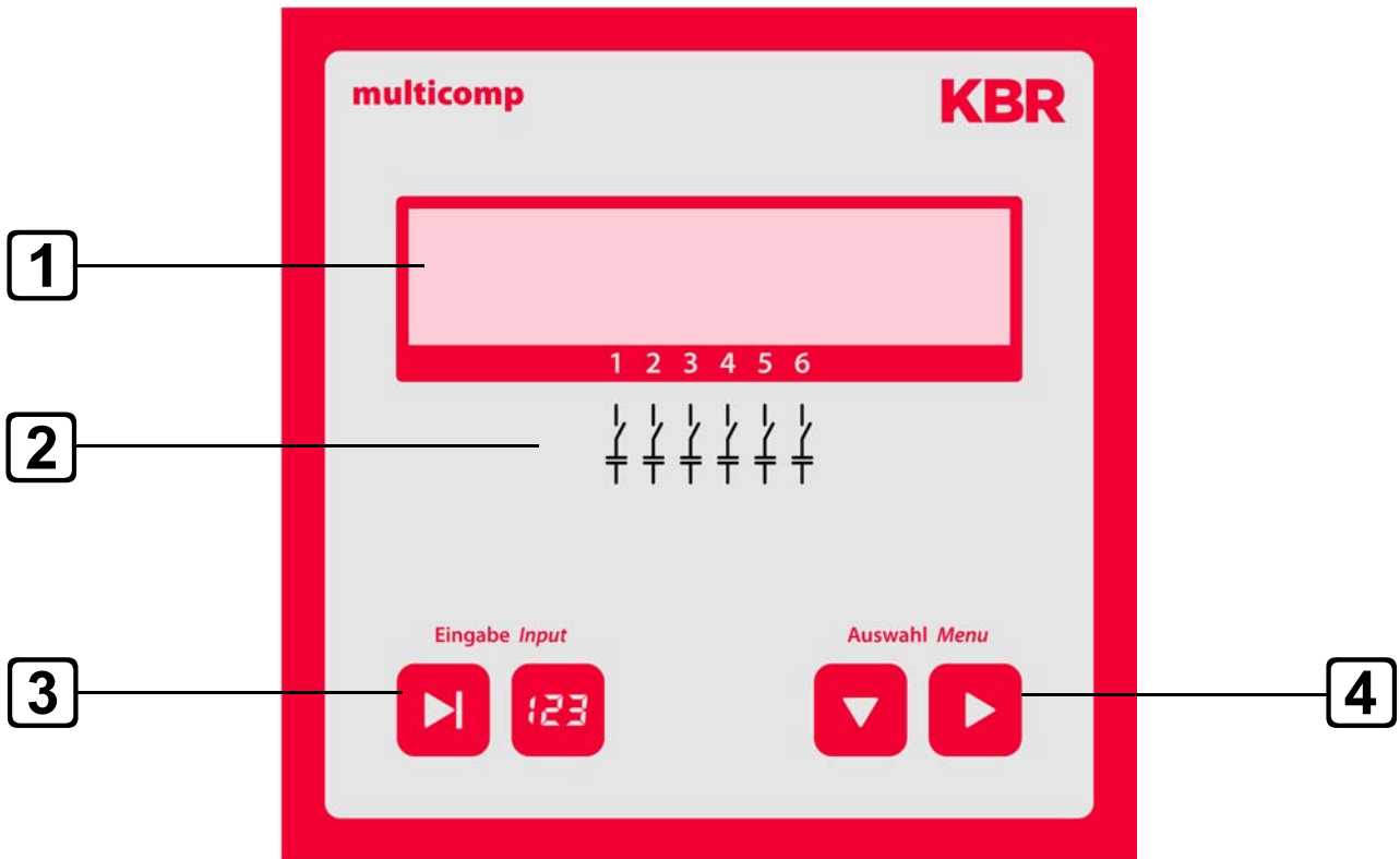
multicom 2F144-NC-1V1C6DO
